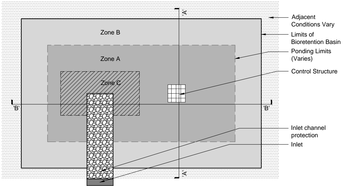
Plan: Zone Widths Vary
