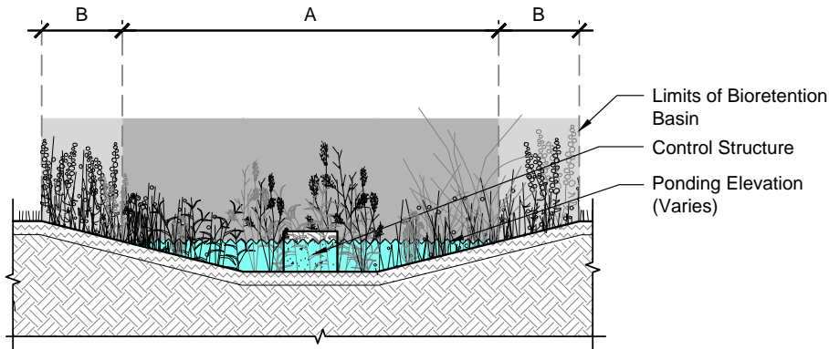
Section 'A-A': Zone Widths Vary
