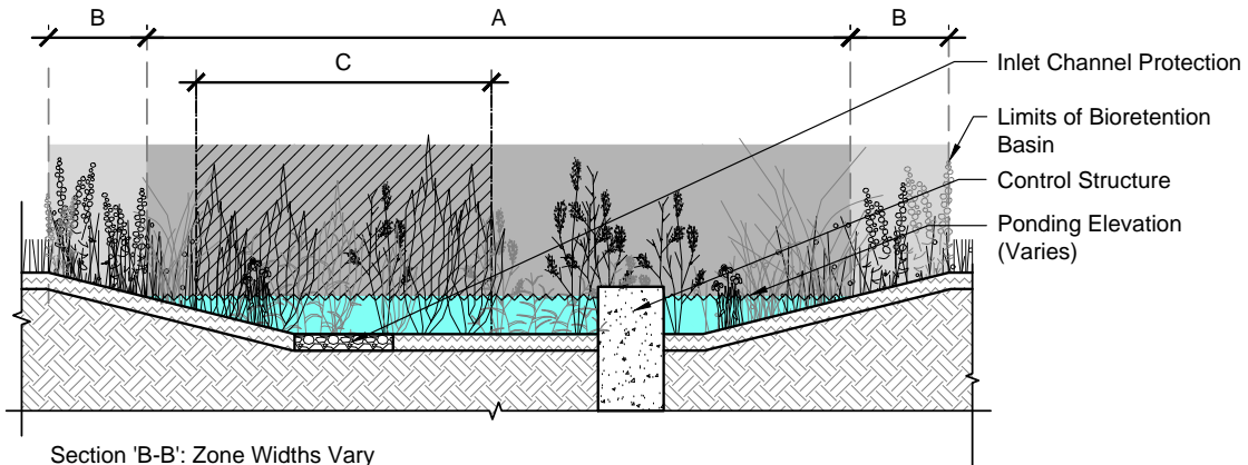
Section 'B-B': Zone Widths Vary
