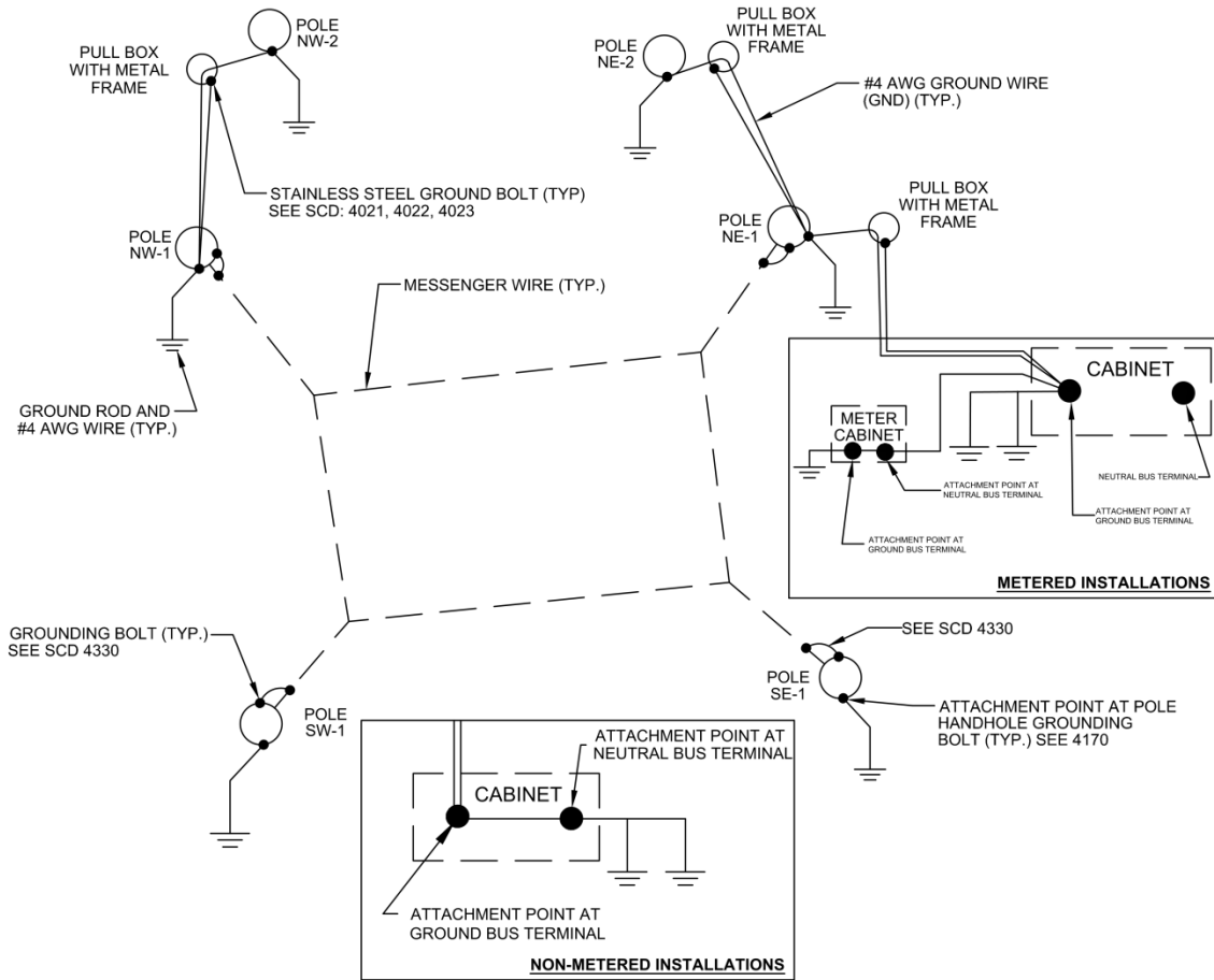
Figure 7.2 Grounding and Bonding Wiring Illustration Span Wire Example
