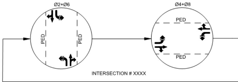
Figure 15.7 2 Phase Example North-South Mainline
