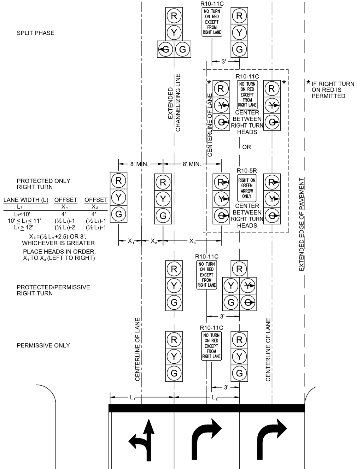
Figure 5.17 Vehicular Signal Head Alignment Three Approach Lanes Configuration G
